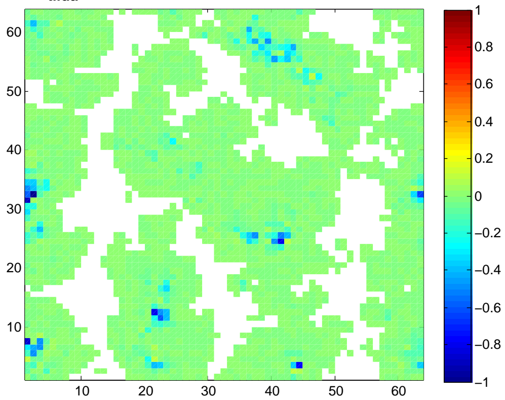
TI_{\text{tilda}} - TI (25th percentile), 1km grid (z=2025m)
