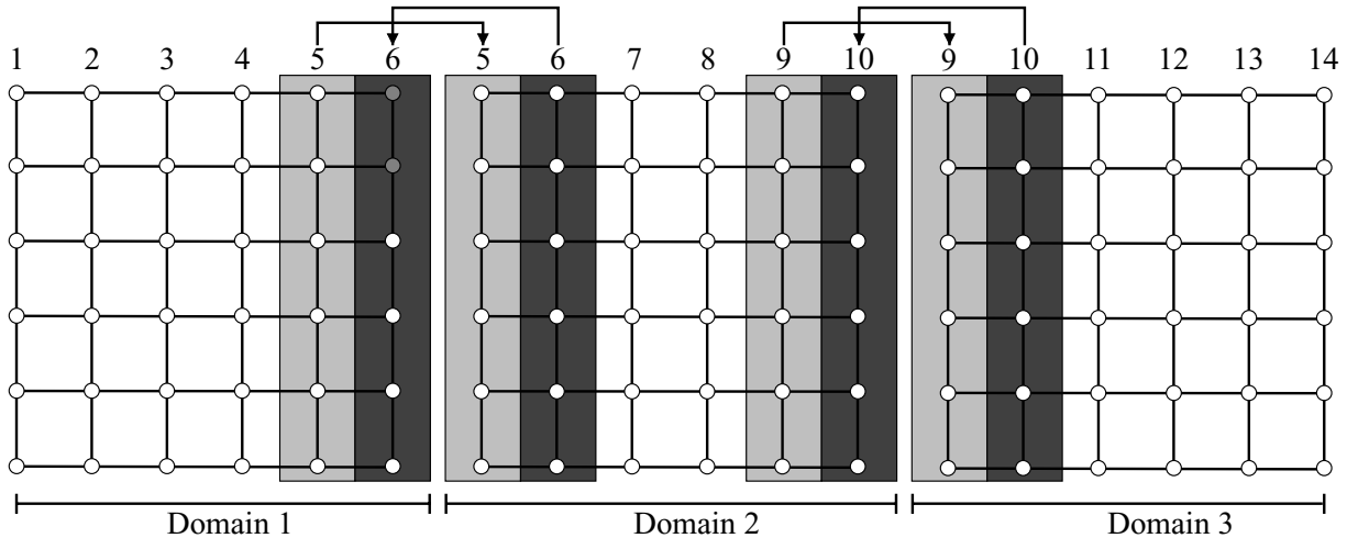
Figure 5. Schematic illustration of the domain decomposition used for parallelization of the SHaxi algorithm. The model space is divided into multiple domains (here shown for three domains) which are each processed by an individual node. After each time step the gridpoints at the boundaries of the domain (gridpoints underlain in grey) are copied to the corresponding gridpoints of the adjacent domain. The lateral size of the grey regions correspond to half the FD operator length.
