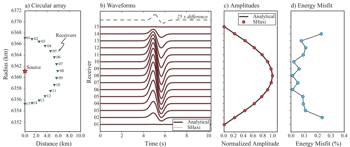
Figure 6. (a) Source–receiver setup of the circular array used to examine the angular variation of the radiation pattern. In this setup the entire range of take-off angle is covered. (b) Numerical FD (red solid line) and analytical (black solid line) seismograms for the array. The dashed line on top shows the difference trace for receiver no. 8 scaled by a factor of 25. (c) The maximum FD amplitudes of all traces (red filled circles) are plotted on top of the analytical curve (solid line). (d) The energy misfit of the FD solution with respect to the analytical solutions. Receivers 01 and 15 are on the nodal SH plane and the energy misfit is undefined. The energy misfit across all receivers is less than 0.3 per cent.
