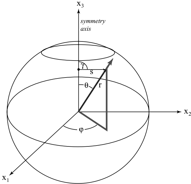
Figure 1. Spherical coordinate system used in the formulation of the wave equation and the source description. All properties are invariant in the \phi -direction. The distance from the Earth's centre is denoted by r , and \theta is the angular distance from the symmetry axis, \gamma is the take-off angle, and s is the source–receiver distance.
