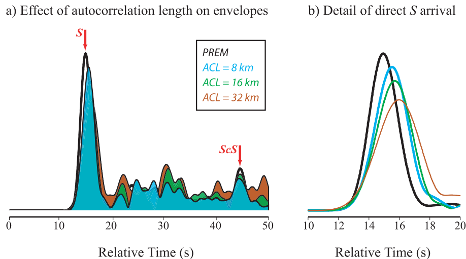
Figure 11. (a) The dependence of autocorrelation length (ACL) on SH -wave envelopes. Envelopes of displacement seismograms are shown for the PREM model (black line) and for the PREM model with three realizations of random S -wave velocity perturbations applied. The perturbations are produced for a Gaussian autocorrelation function with 3 per cent rms velocity perturbations. Envelopes are shown for random perturbations with ACL's of 8 km (blue), 16 km (green) and 32 km (red). (b) Detail of direct S arrival from panel (a).
