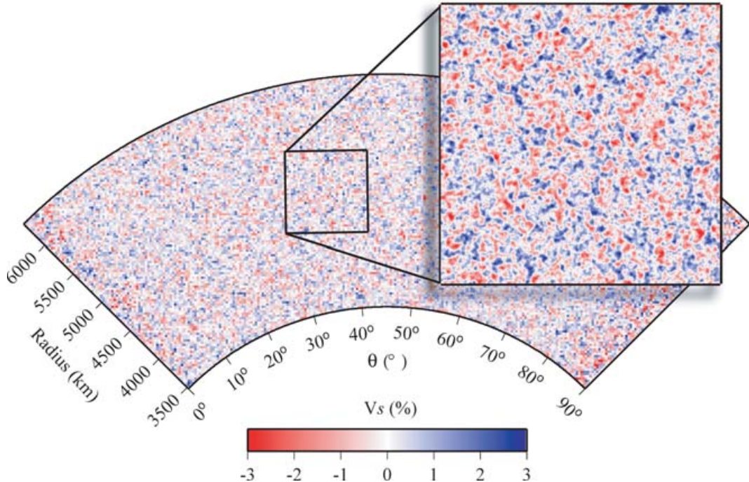
Figure 8. Example of SHaxi model for which random V_S variations were applied to the PREM background model. In this example a Gaussian autocorrelation function was applied with a corner correlation length of 32 km. The rms S -wave velocity perturbation is 1 per cent and the maximum perturbation varies between \pm 3 per cent. The left model boundary at \theta = 0^\circ is the symmetry axis.
