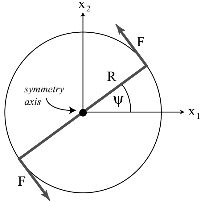
Figure 3. Illustration of the ring source used in the SHaxi algorithm. The origin of the coordinate system corresponds to the symmetry axis. The ring source can be thought as a superposition of single forces F acting perpendicular to the radius vector R(\psi) .
