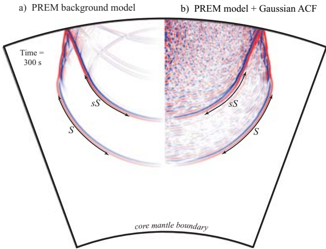
Figure 9. (a) The SH velocity wavefield for a 200-km-deep source in the PREM background model at time = 300 s. The S and sS wave fronts are labelled. (b) The velocity wavefield at the same time step as in panel (a) for the PREM model with random V_S variations applied. The random variations were created with a Gaussian autocorrelation function with corner wavelength of 32 km and 3 per cent rms V_S perturbations.
