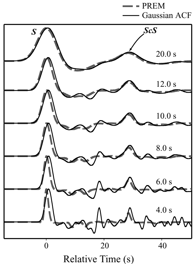
Figure 10. Frequency dependence of scattering. Shown are SHaxi displacement seismograms for the PREM earth model (dashed line) compared to seismograms for a stochastically perturbed model with a Gaussian autocorrelation function created with a rms V_S perturbation of 3 per cent and a 16 km corner correlation length superimposed on PREM (solid line). Each pair of seismograms has been filtered to a different dominant period listed directly above the seismogram pair. Seismograms are normalized to unity on the S arrival.
