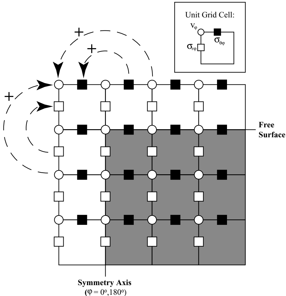
Figure 4. Detail of the top left-hand corner of the SHaxi grid where the free surface and symmetry boundaries are encountered. The interior gridpoints (region underlain in grey) are part of the physical model space. To fulfil the boundary conditions, gridpoints outside of the physical model space (region not underlain in grey) must be added to the total grid. These outer points are updated at each time step by corresponding values of grid elements inside the physical model space, as indicated by the arrows and the plus (+) and minus (−) symbols.
