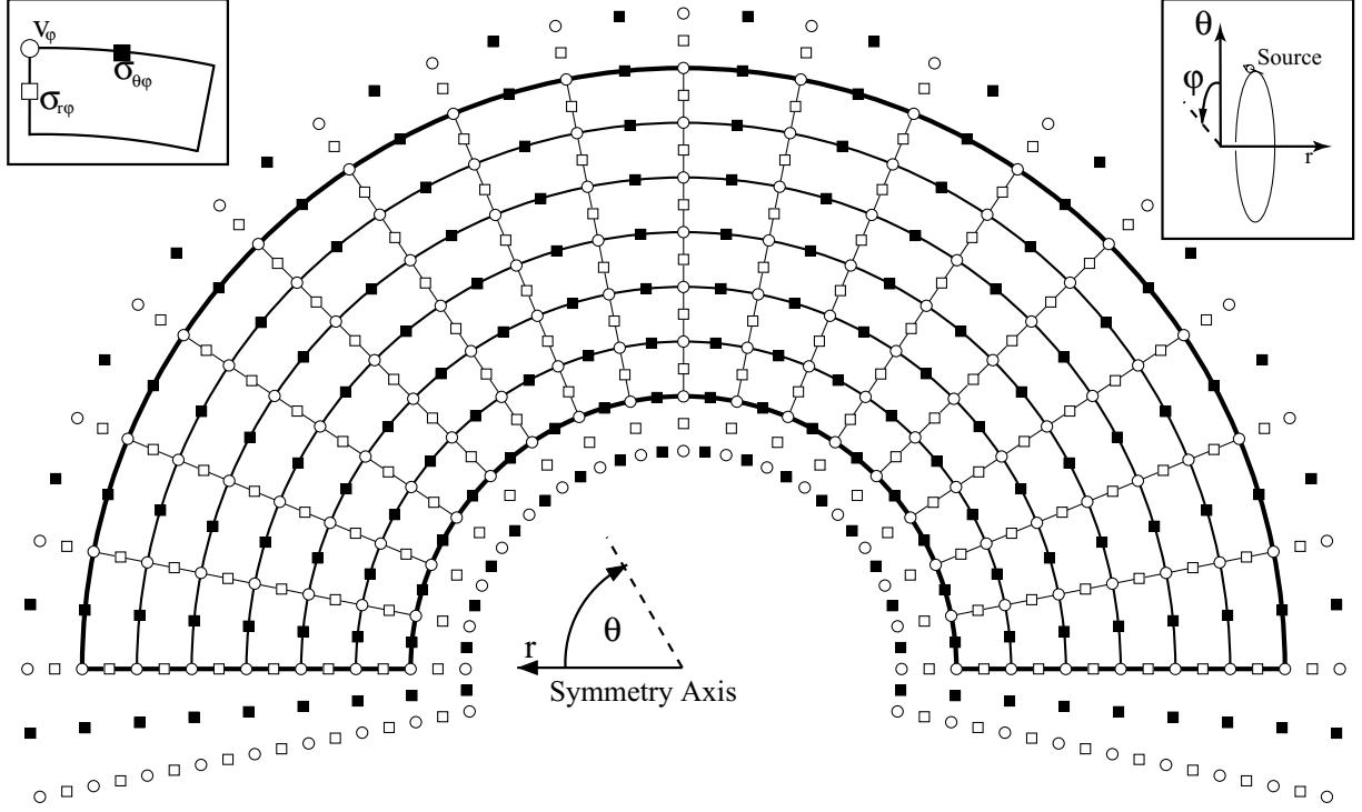
Figure 2. The staggered grid scheme used in the SHaxi algorithm. The origin of the coordinate system is placed at the Earth's centre. The symmetry axis ( \theta = 0^\circ ) is horizontally aligned as labelled at the origin. The model boundaries (surface, CMB and symmetry axis) are framed with thick lines. The additional points outside the model space are used for implementation of the boundary conditions. The symbols representing the wavefield properties v_\varphi , \sigma_{r\varphi} and \sigma_{\theta\varphi} are labelled in the unit grid-cell shown in the top left corner of the figure.
