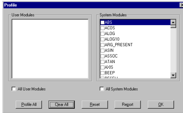
Figure 12-4: Profile Dialog
