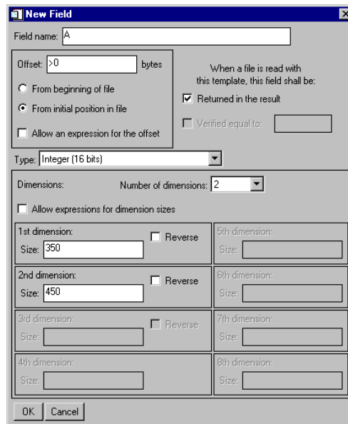
Figure 3-7: Modifying fields in binary template
