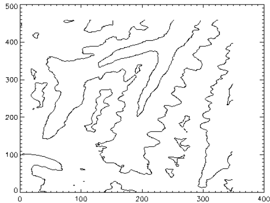
Figure 7-7: Contour plot
