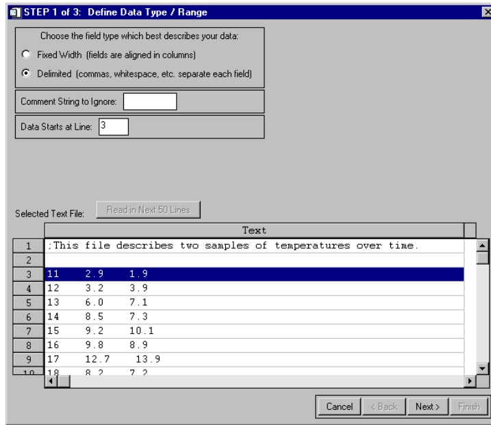
Figure 3-2: the ASCII_TEMPLATE dialog
