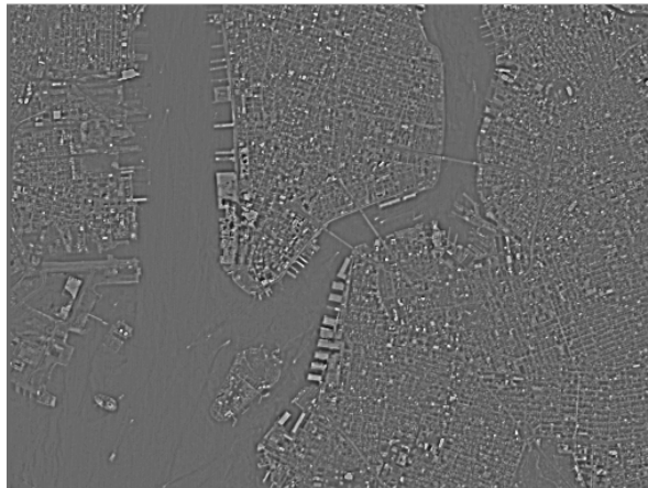
Figure 6-12: Unsharp masking
