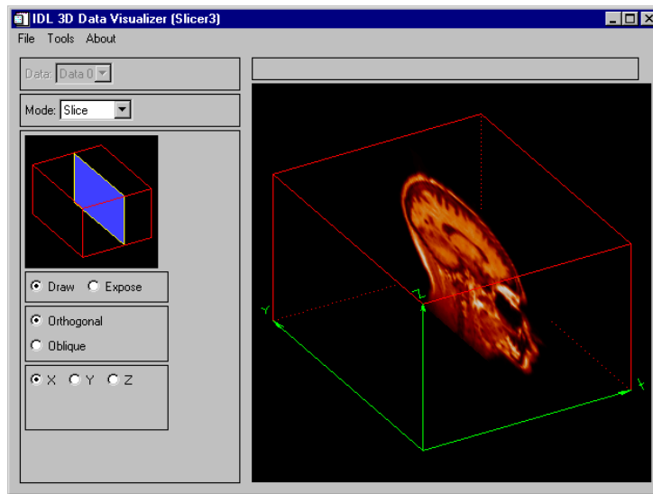
Figure 8-3: IDL Slicer3
