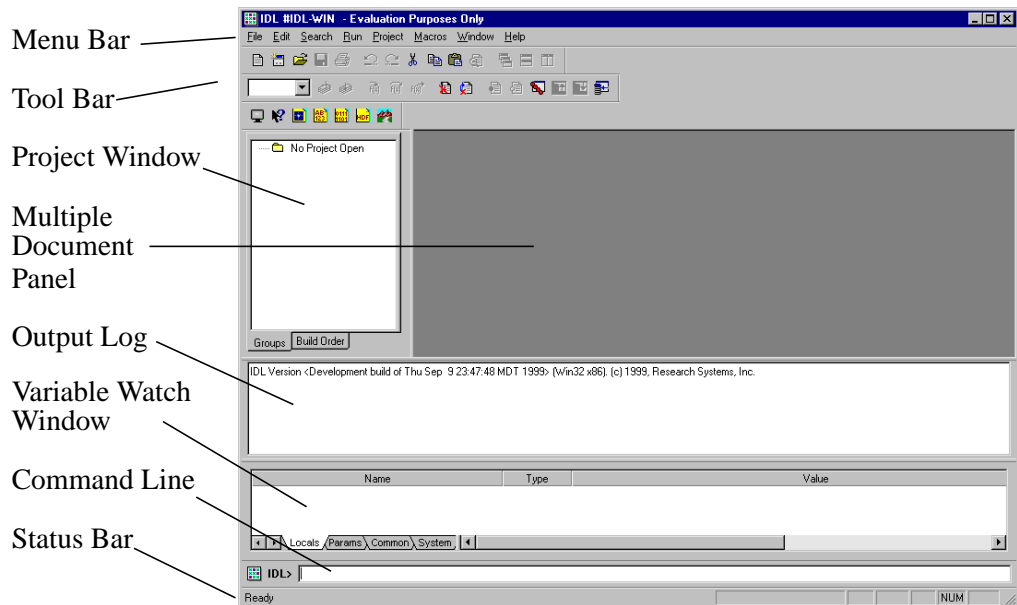
Figure 2-1: The IDL Development Environment for Windows
