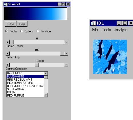
Figure 14-4: The GUI window with mineral.gif loaded (right) and the color table (left)
