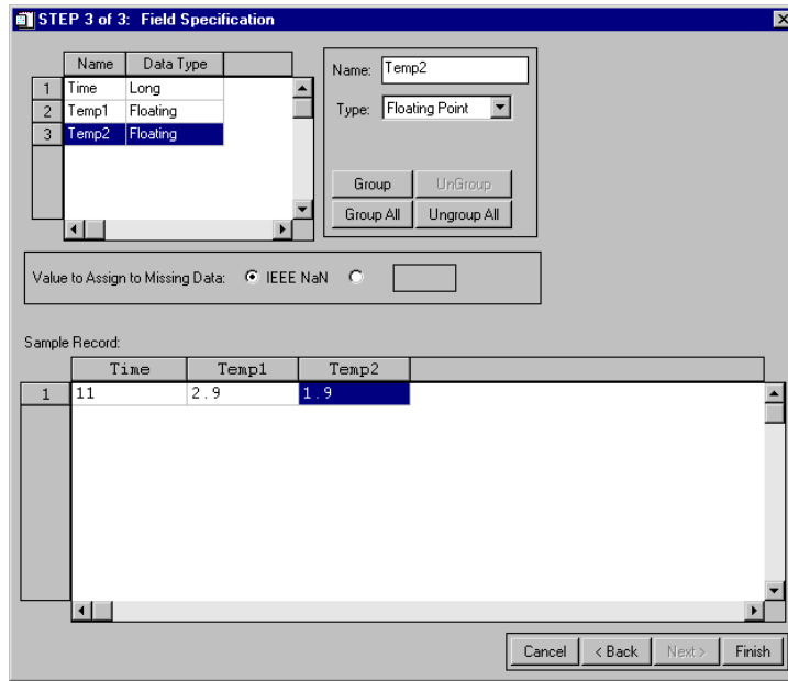
Figure 3-4: Naming the data type sets in ASCII_TEMPLATE
