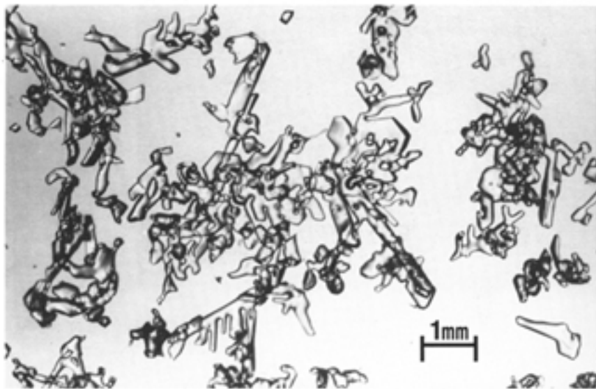
Class 2dc, partly decomposed precipitation particles. Photo by E. Akitaya.
