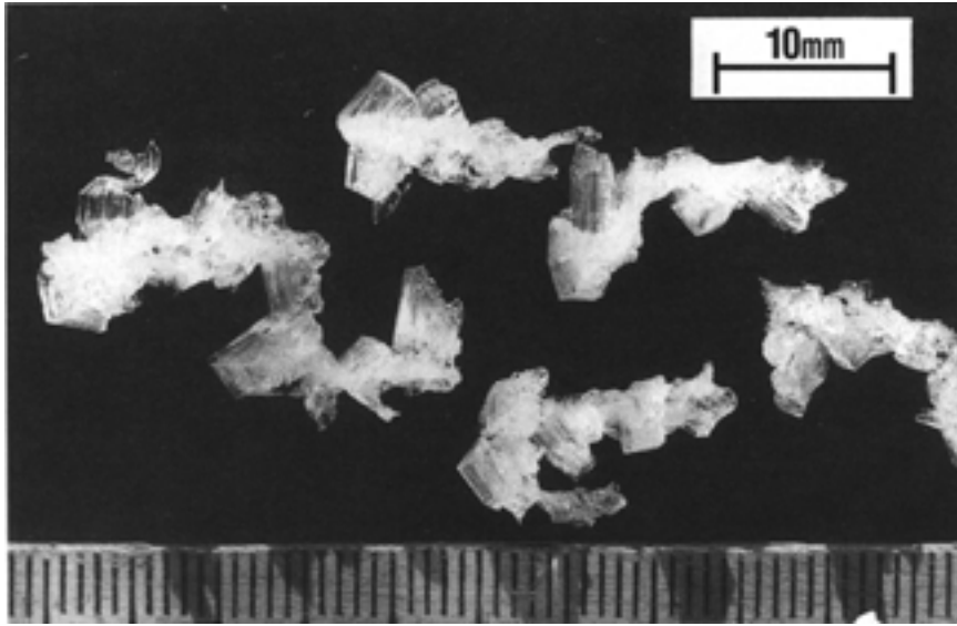
Class 5dh, cup-shaped crystals arranged in columns. Photo by E. Akitaya.
