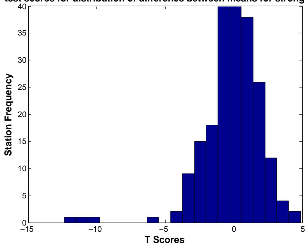
T test scores for distribution of difference between means for strong fronts
