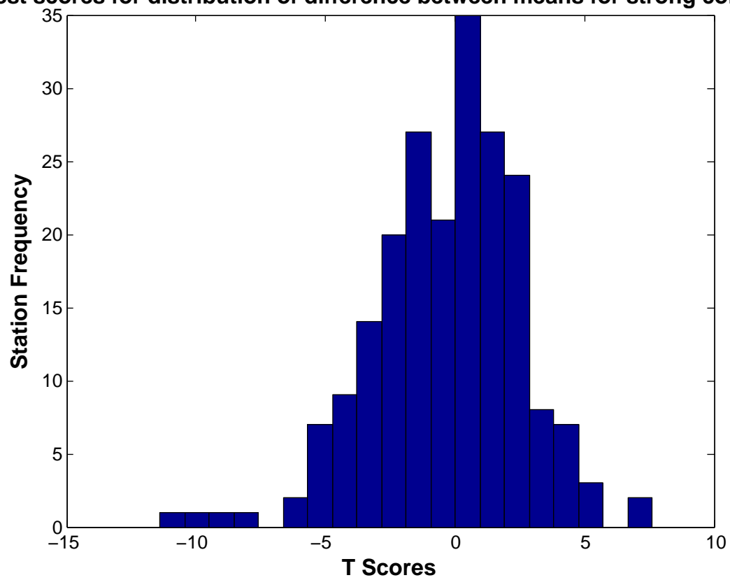
T test scores for distribution of difference between means for strong cold poo
