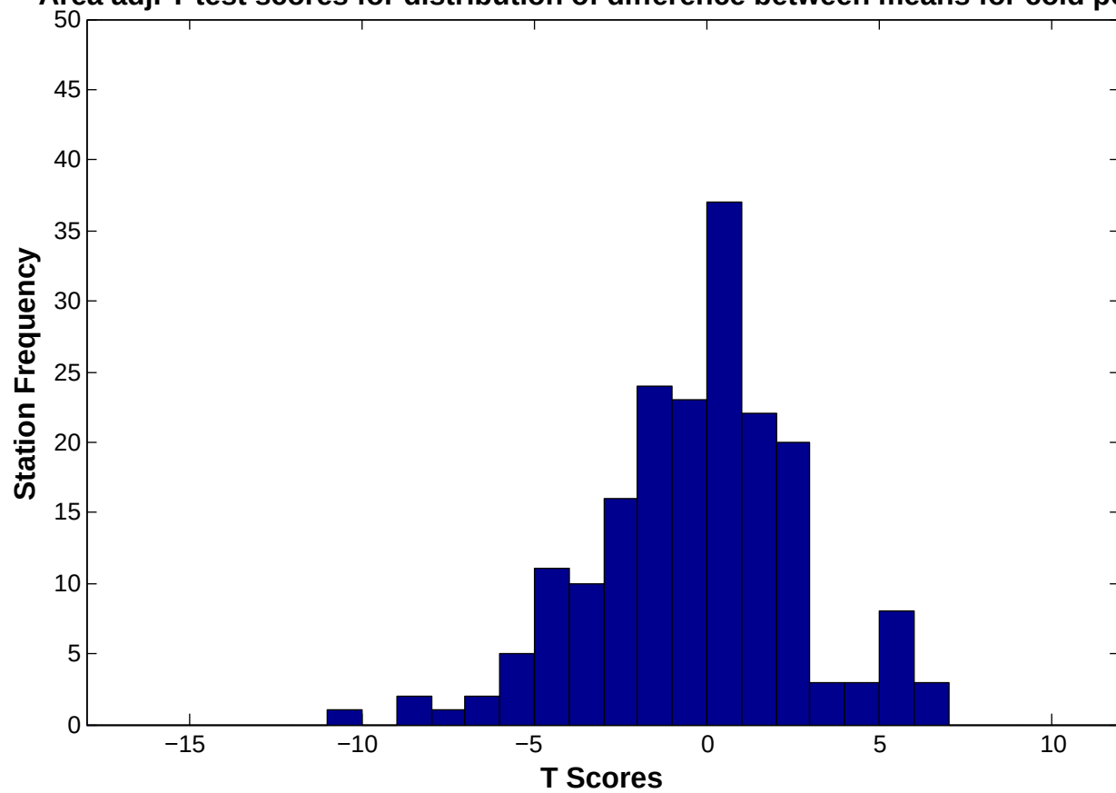
Area adj. T test scores for distribution of difference between means for cold pools
