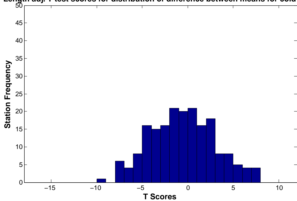
Length adj. T test scores for distribution of difference between means for cold pools
