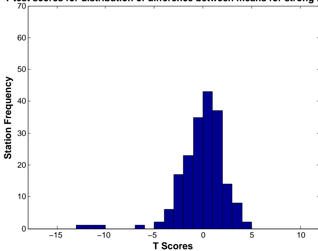
T test scores for distribution of difference between means for strong fronts
