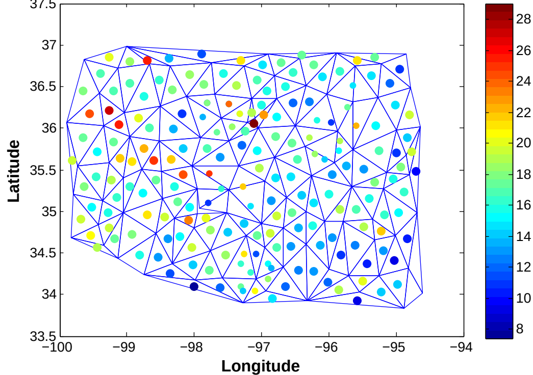
Annual Frontal Passage Frequency (Area Adjusted) with cold pools
