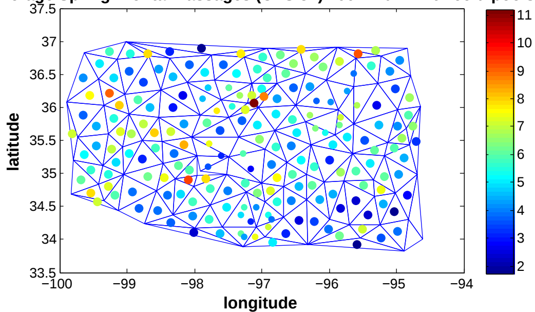
Average Spring Frontal Passages (CPS 3+) 1997–2011 with cold pools
