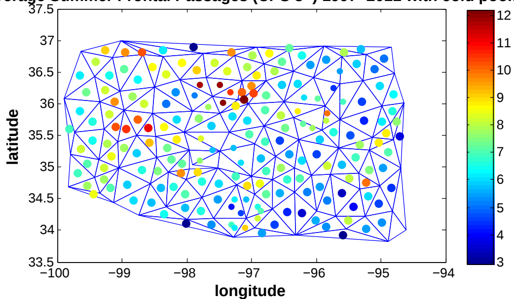
Average Summer Frontal Passages (CPS 3+) 1997–2011 with cold pools
