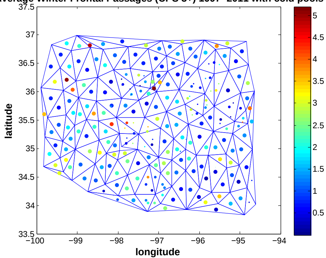
Average Winter Frontal Passages (CPS 3+) 1997–2011 with cold pools
