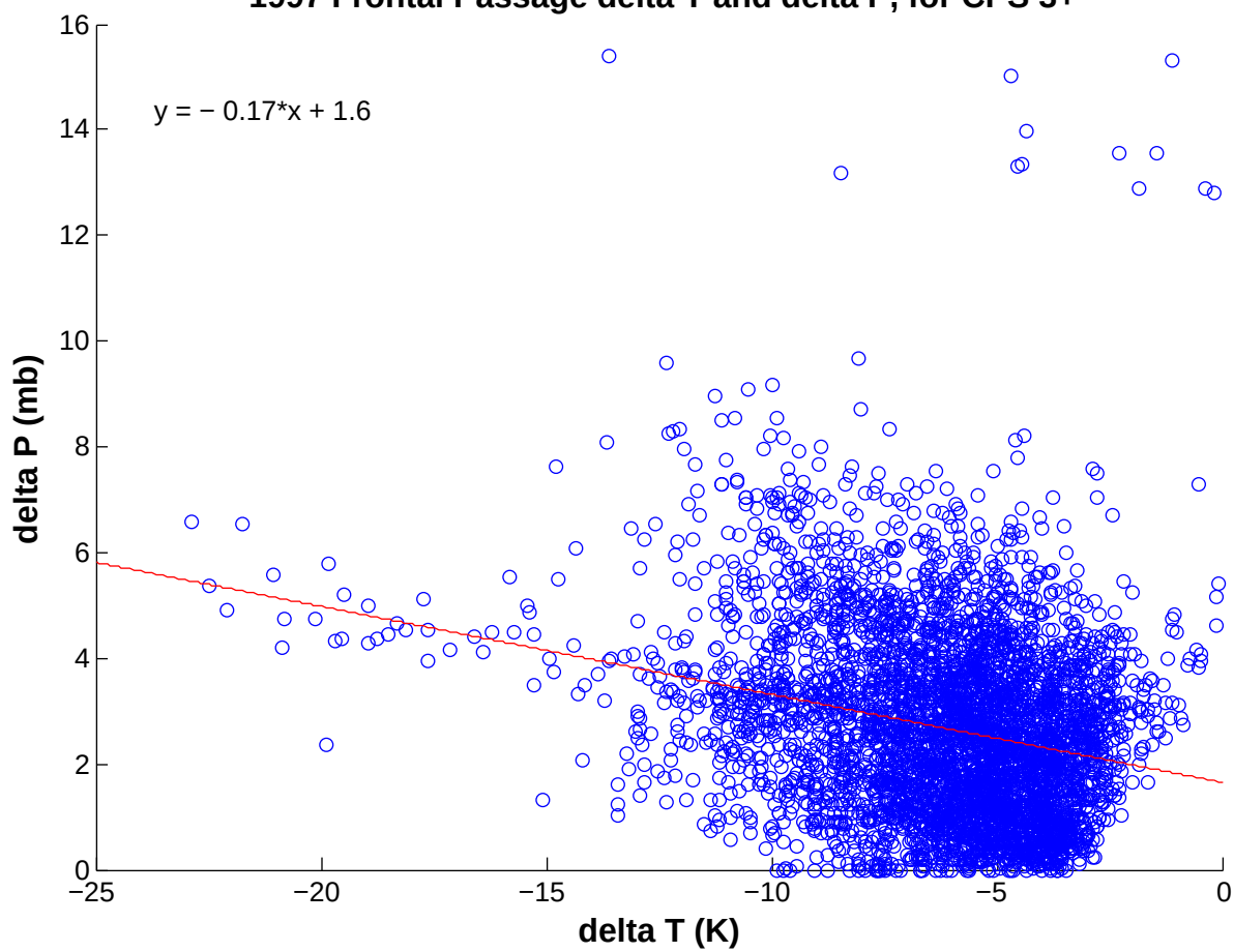
1997 Frontal Passage delta T and delta P, for CPS 3+
