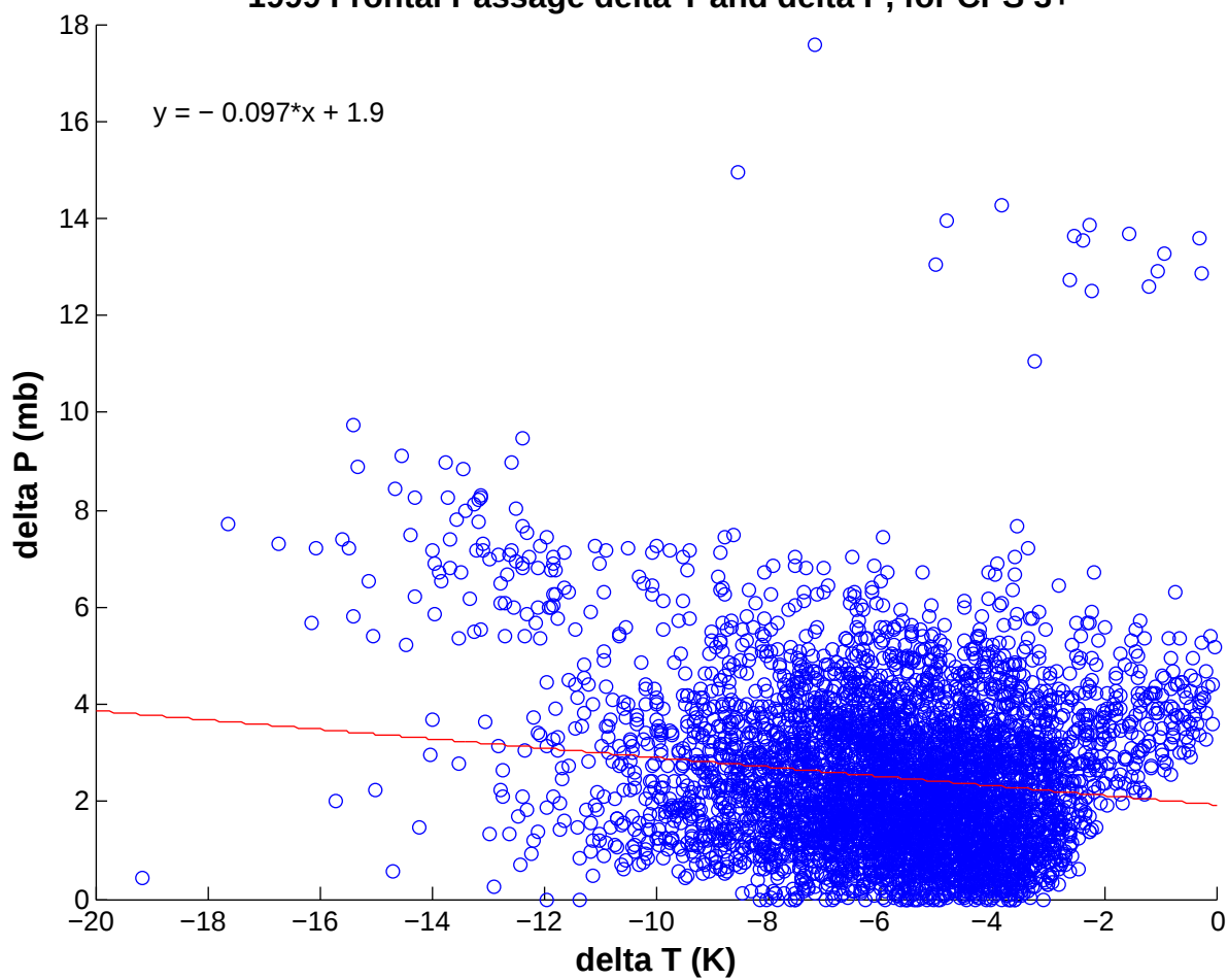
1999 Frontal Passage delta T and delta P, for CPS 3+
