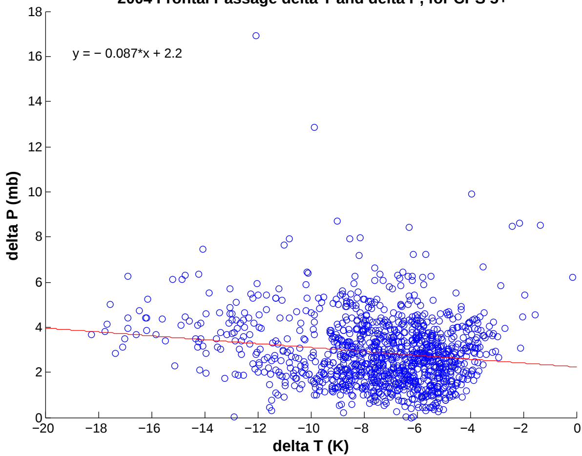
2004 Frontal Passage delta T and delta P, for CPS 5+
