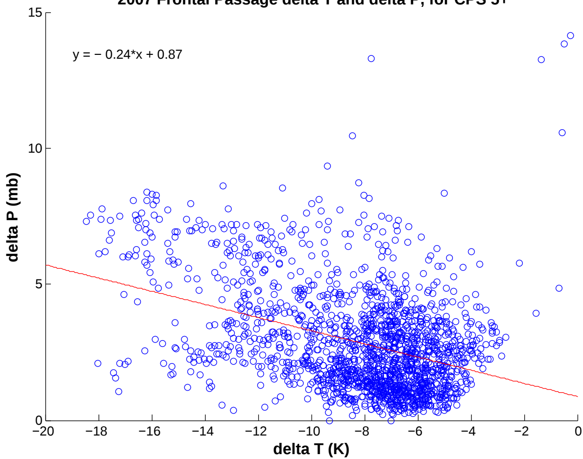
2007 Frontal Passage delta T and delta P, for CPS 5+
