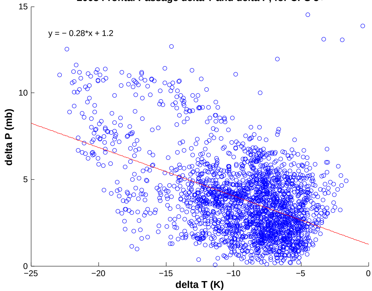
2008 Frontal Passage delta T and delta P, for CPS 5+
