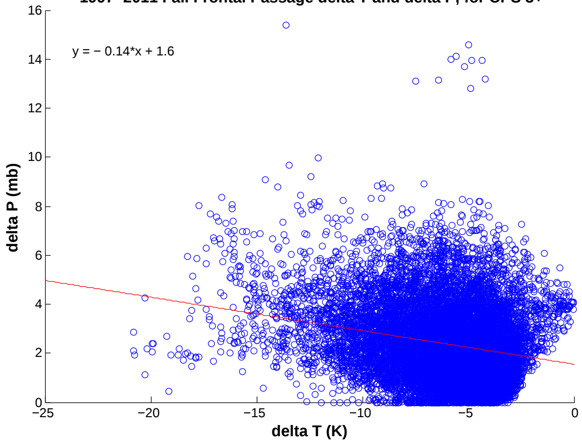
1997–2011 Fall Frontal Passage delta T and delta P, for CPS 3+
