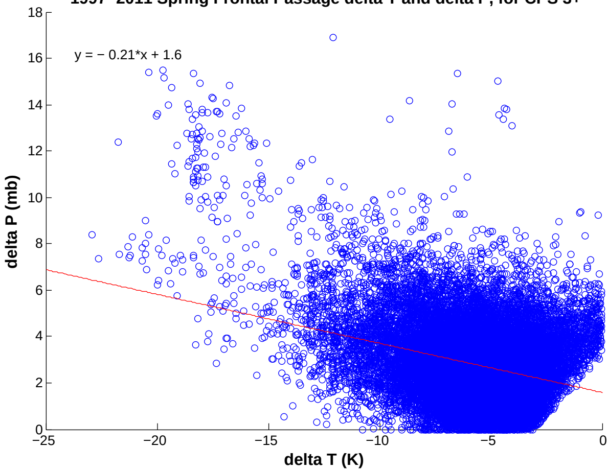
1997–2011 Spring Frontal Passage delta T and delta P, for CPS 3+
