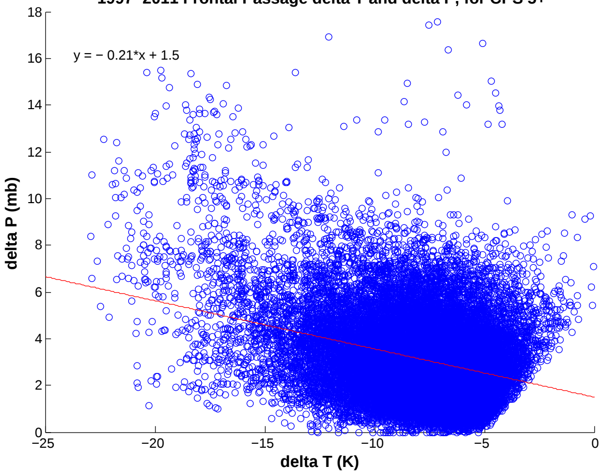
1997–2011 Frontal Passage delta T and delta P, for CPS 5+
