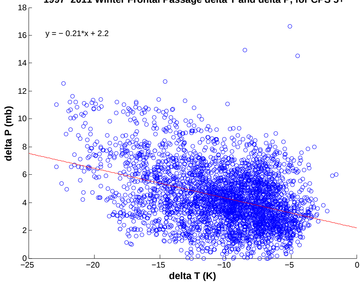
1997–2011 Winter Frontal Passage delta T and delta P, for CPS 5+
