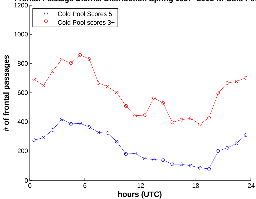
Frontal Passage Diurnal Distribution Spring 1997–2011 w/ Cold Pools
