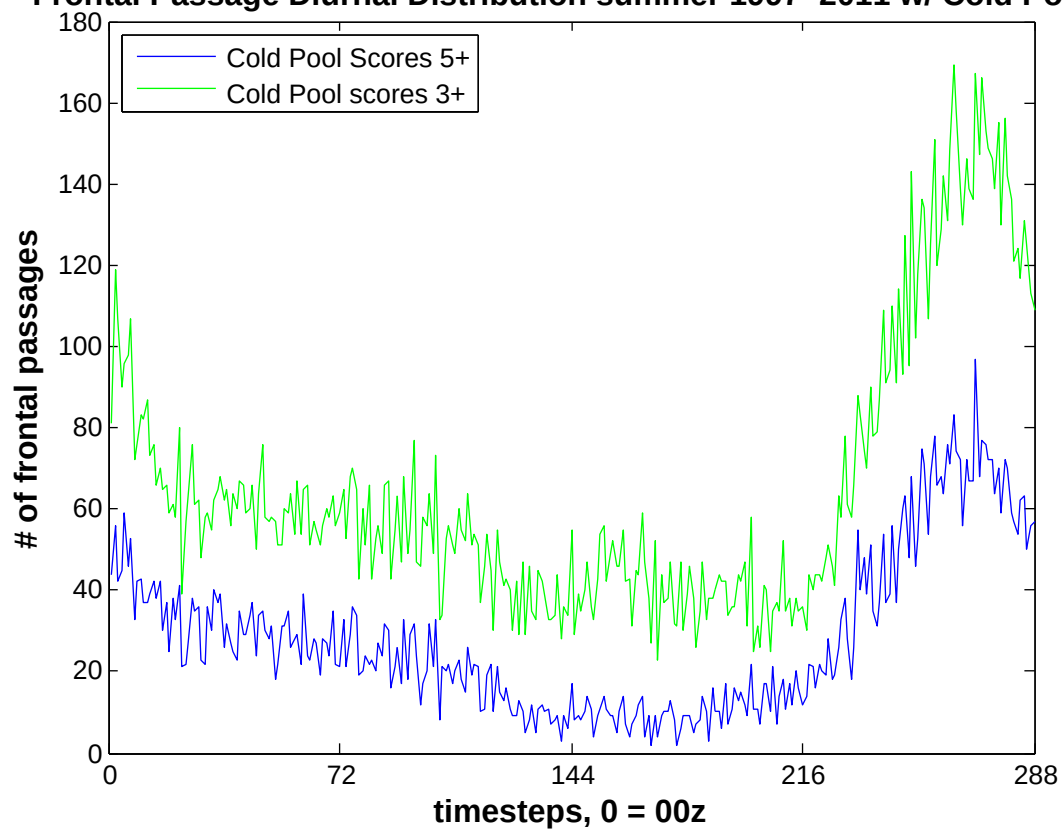
Frontal Passage Diurnal Distribution summer 1997–2011 w/ Cold Pools
