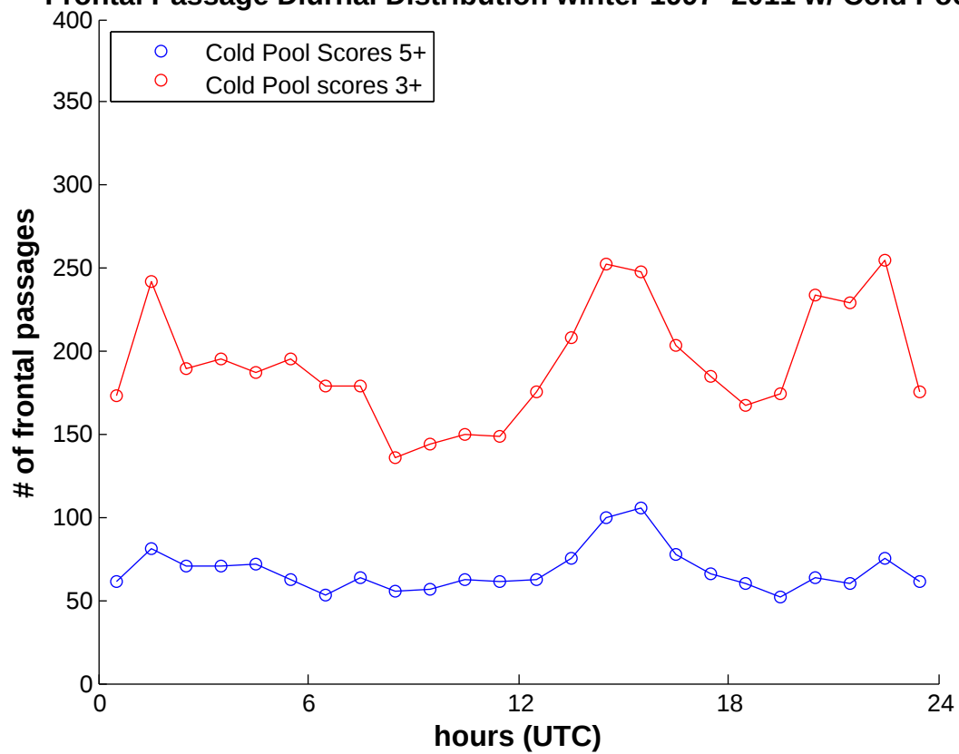
Frontal Passage Diurnal Distribution winter 1997–2011 w/ Cold Pools
