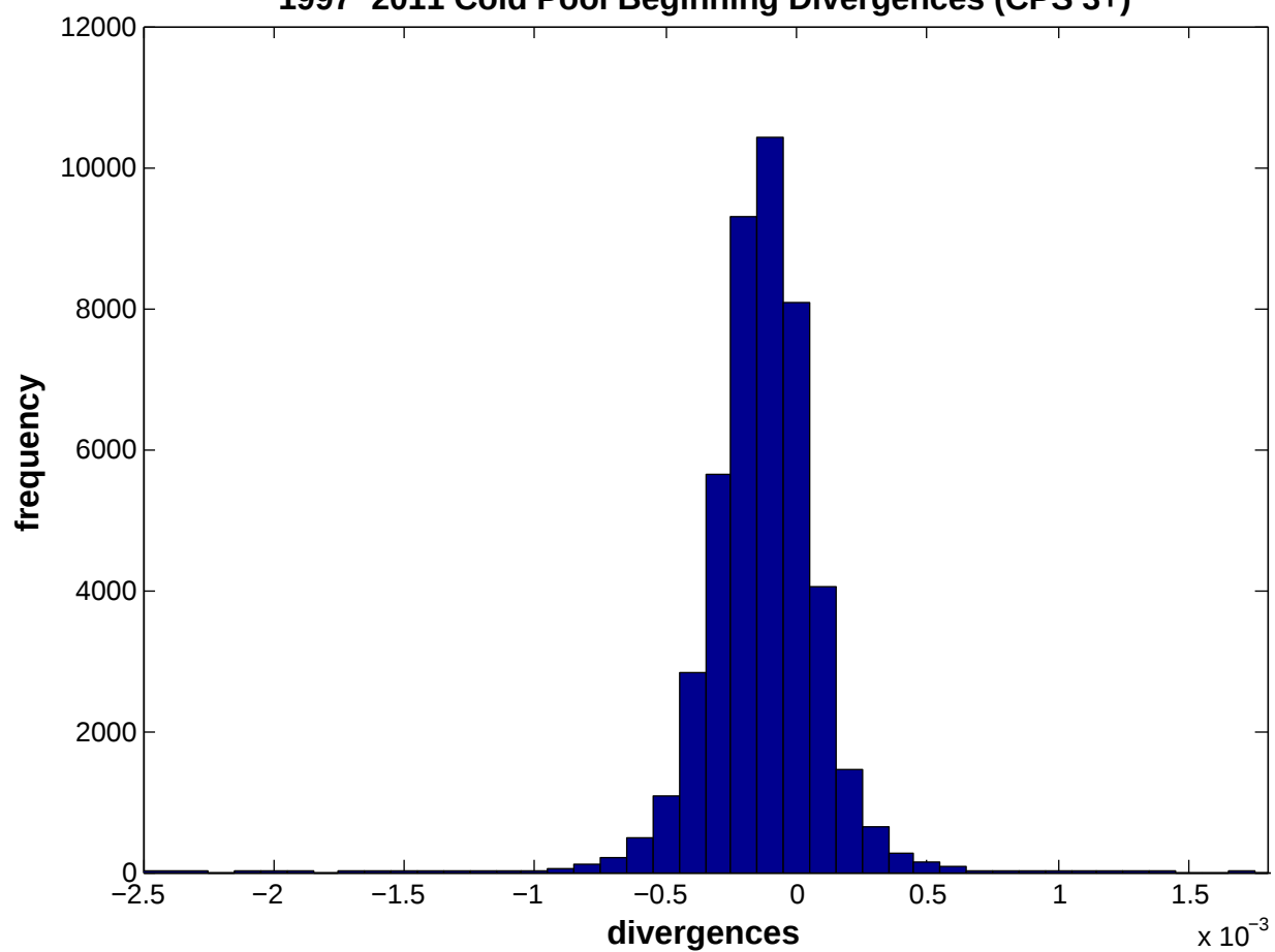
1997–2011 Cold Pool Beginning Divergences (CPS 3+)
