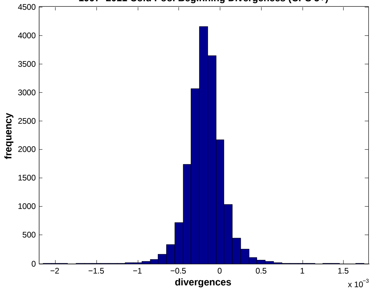
1997–2011 Cold Pool Beginning Divergences (CPS 5+)
