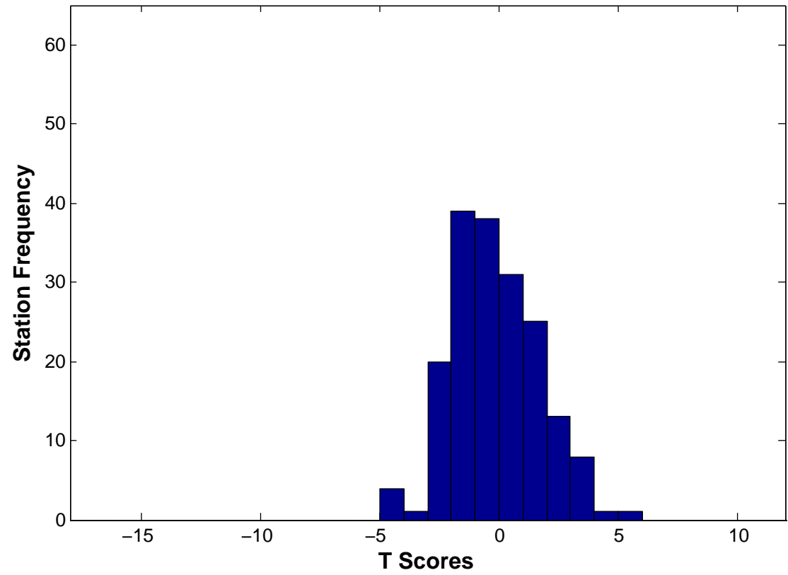
Length adj. T test scores for distribution of difference between means for fronts
