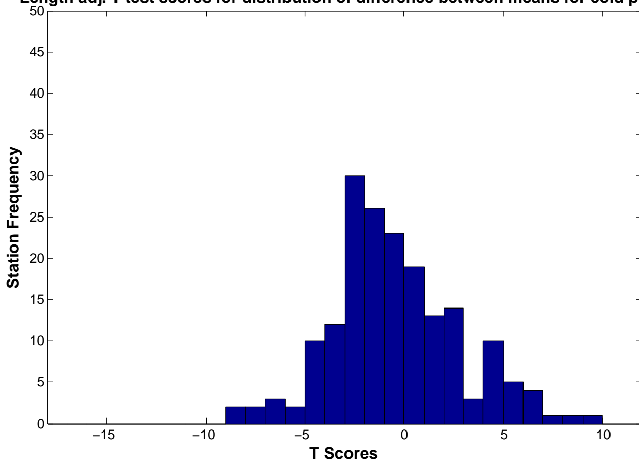
Length adj. T test scores for distribution of difference between means for cold pools
