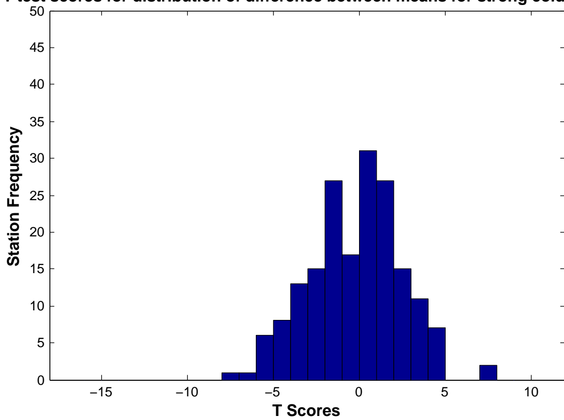
T test scores for distribution of difference between means for strong cold pools
