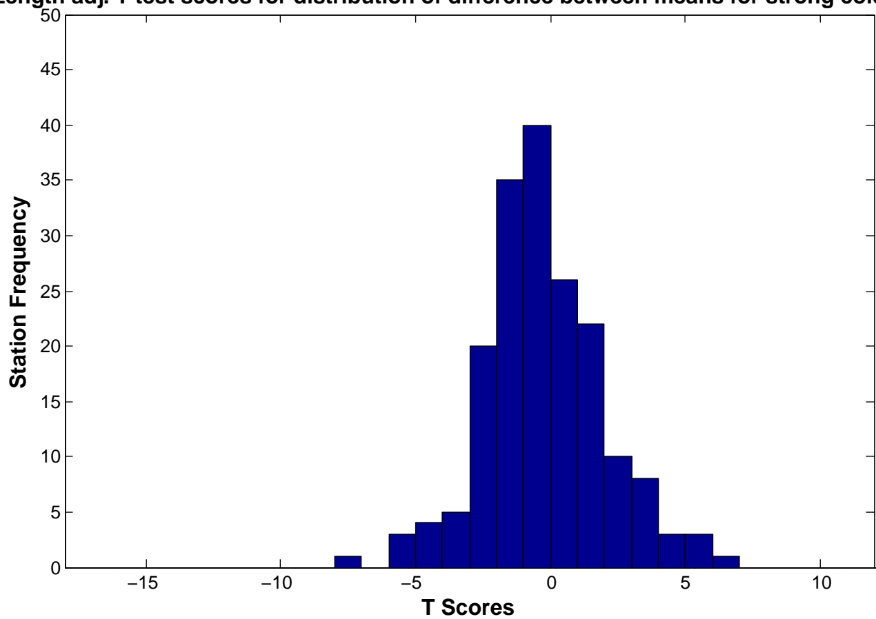
Length adj. T test scores for distribution of difference between means for strong cold pools
