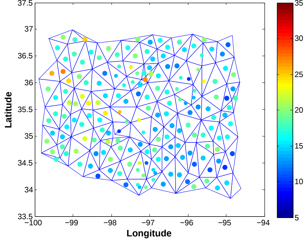
Annual Frontal Passage Frequency (Area Adjusted) with cold pools
