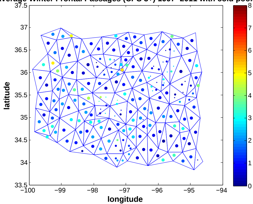
Average Winter Frontal Passages (CPS 3+) 1997–2011 with cold pools
