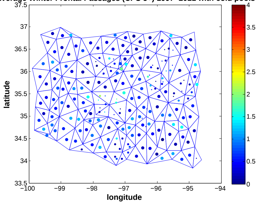
Average Winter Frontal Passages (CPS 5+) 1997–2011 with cold pools
