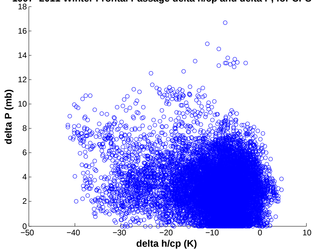
1997–2011 Winter Frontal Passage delta h/cp and delta P, for CPS 3+
