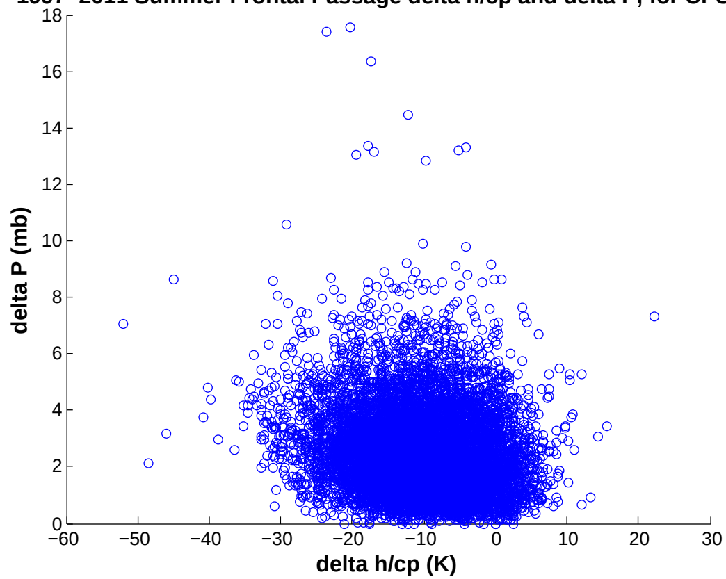
1997–2011 Summer Frontal Passage delta h/cp and delta P, for CPS 5+
