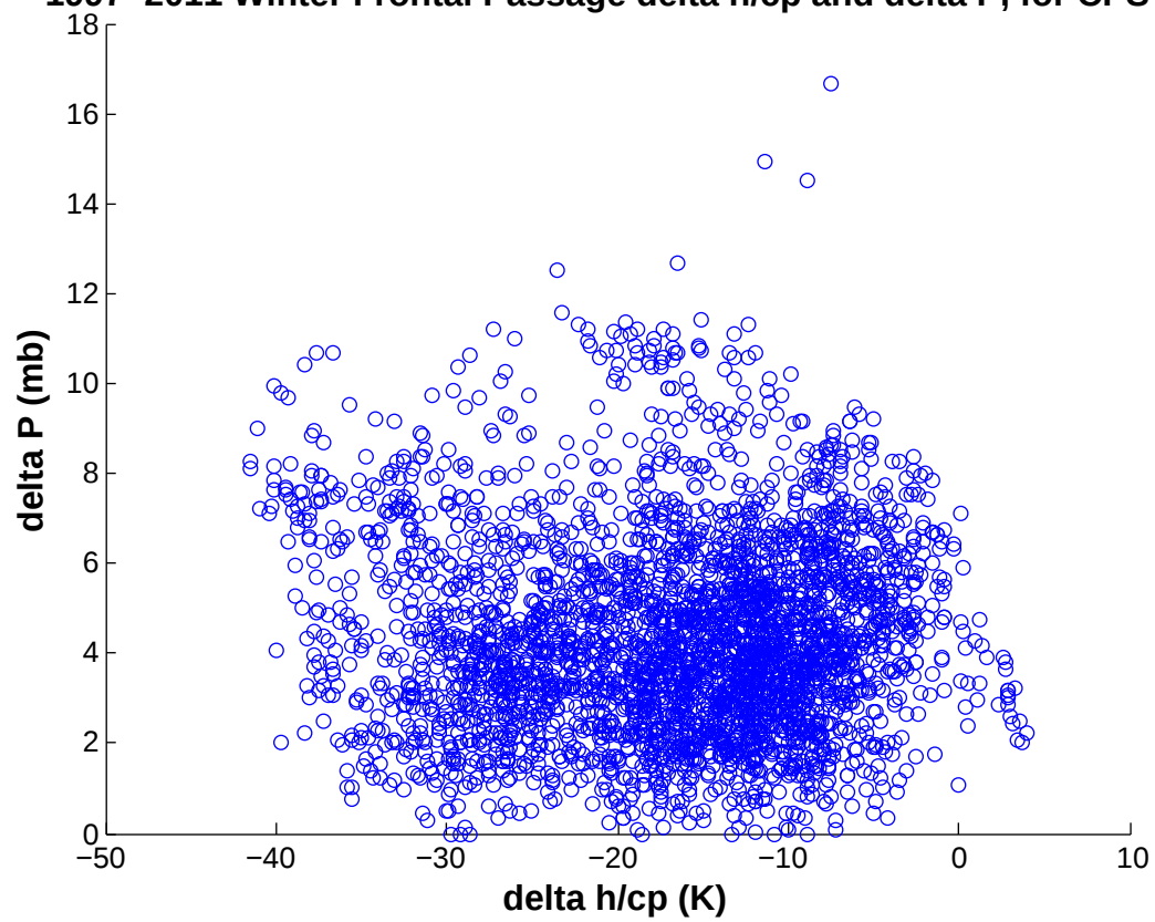
1997–2011 Winter Frontal Passage delta h/cp and delta P, for CPS 5+
