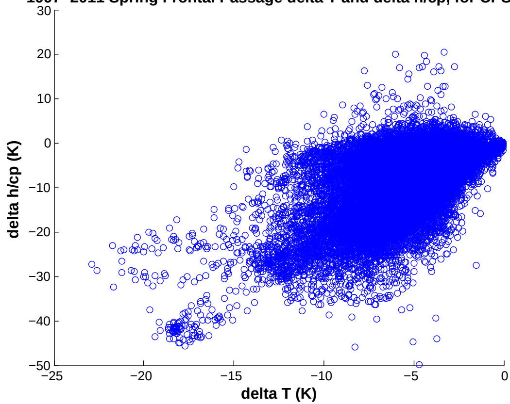
1997–2011 Spring Frontal Passage delta T and delta h/cp, for CPS 3+
