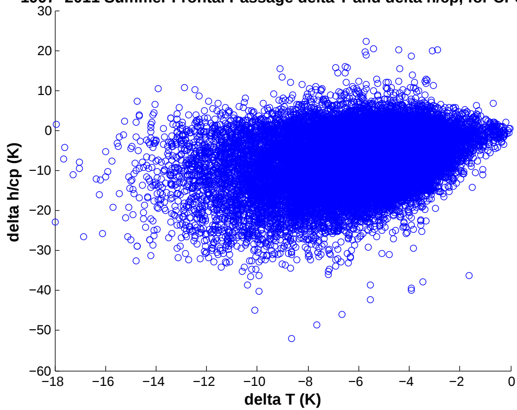
1997–2011 Summer Frontal Passage delta T and delta h/cp, for CPS 3+
