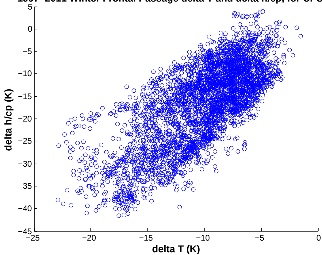
1997–2011 Winter Frontal Passage delta T and delta h/cp, for CPS 5+
