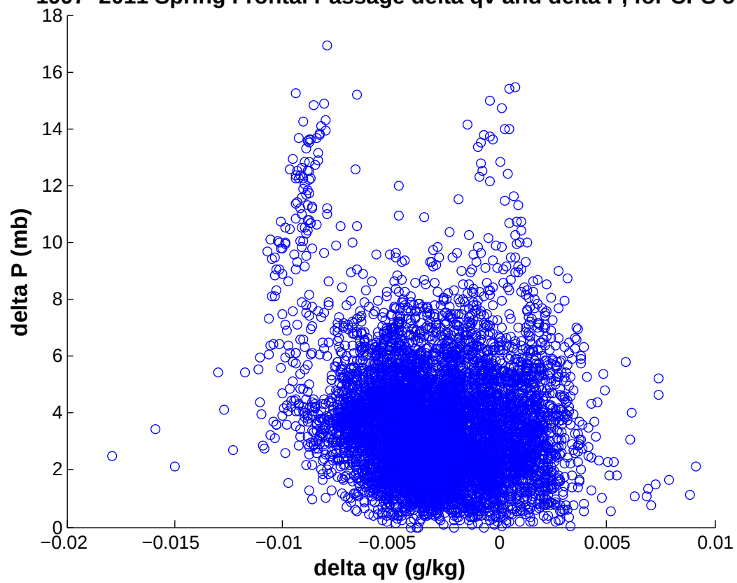
1997–2011 Spring Frontal Passage delta qv and delta P, for CPS 5+
