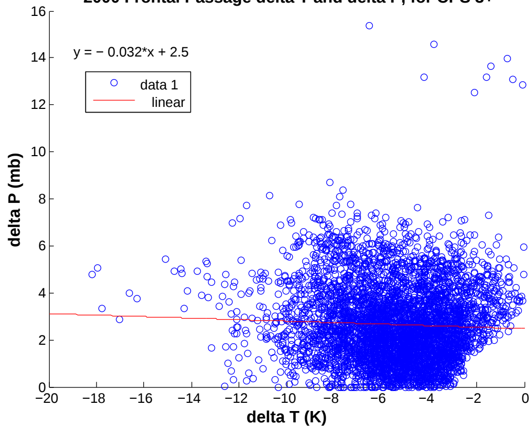
2000 Frontal Passage delta T and delta P, for CPS 3+
