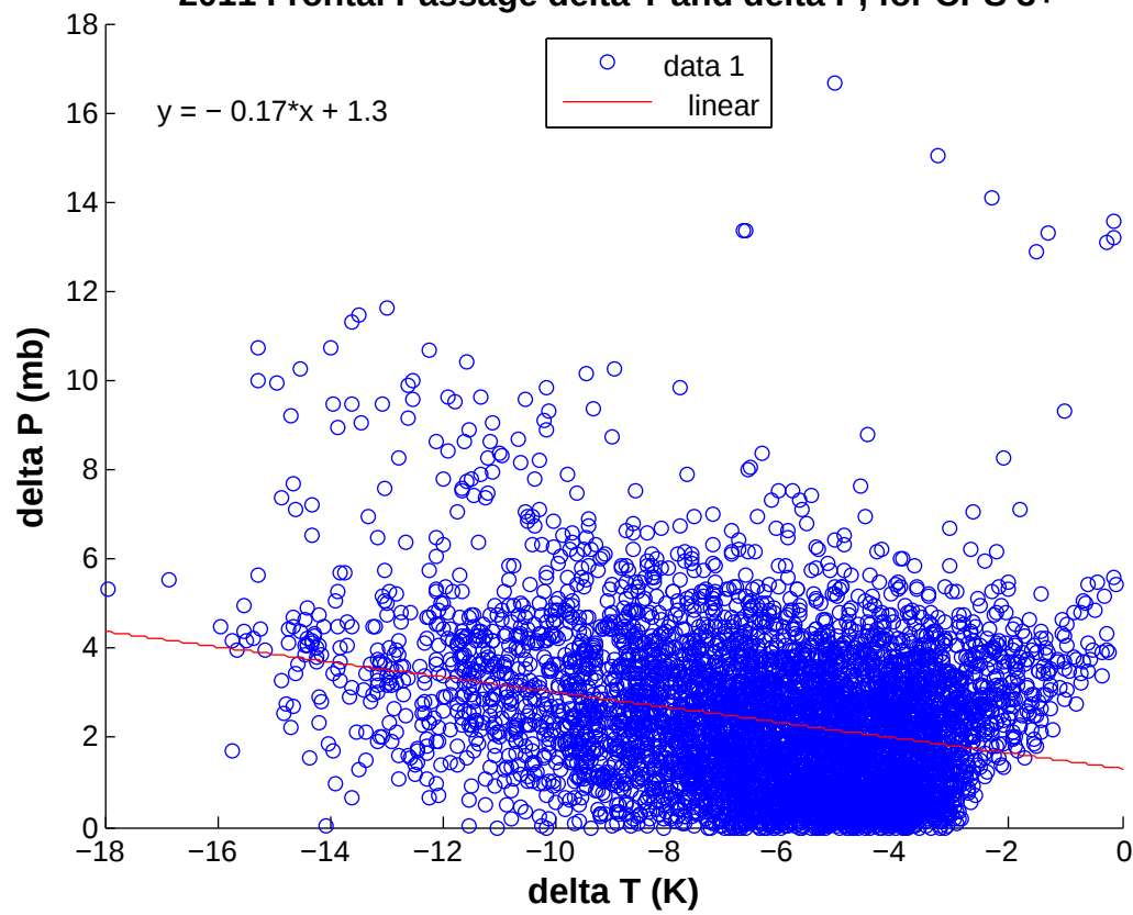
2011 Frontal Passage delta T and delta P, for CPS 3+
