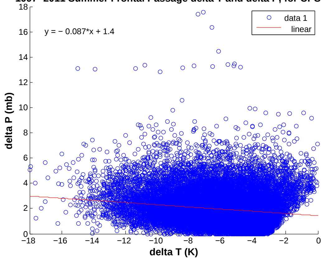
1997–2011 Summer Frontal Passage delta T and delta P, for CPS 3+
