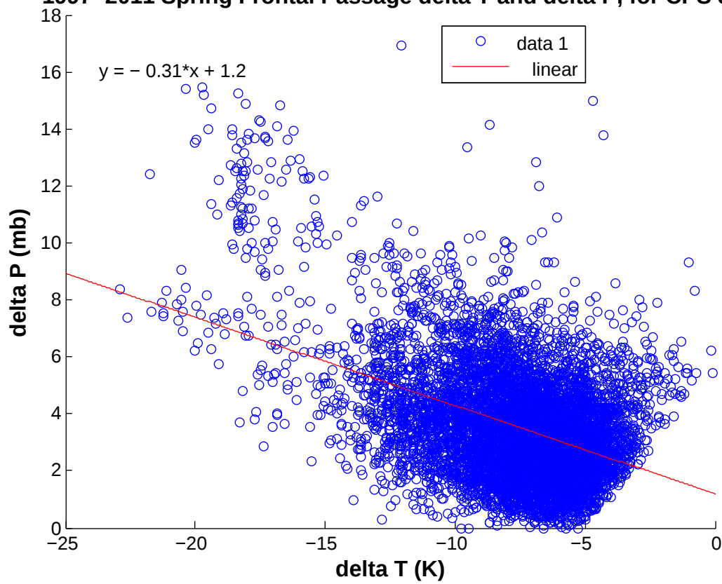
1997–2011 Spring Frontal Passage delta T and delta P, for CPS 5+
