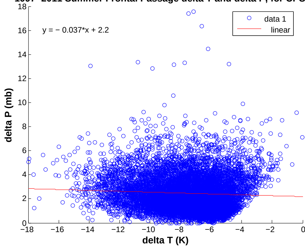
1997–2011 Summer Frontal Passage delta T and delta P, for CPS 5+
