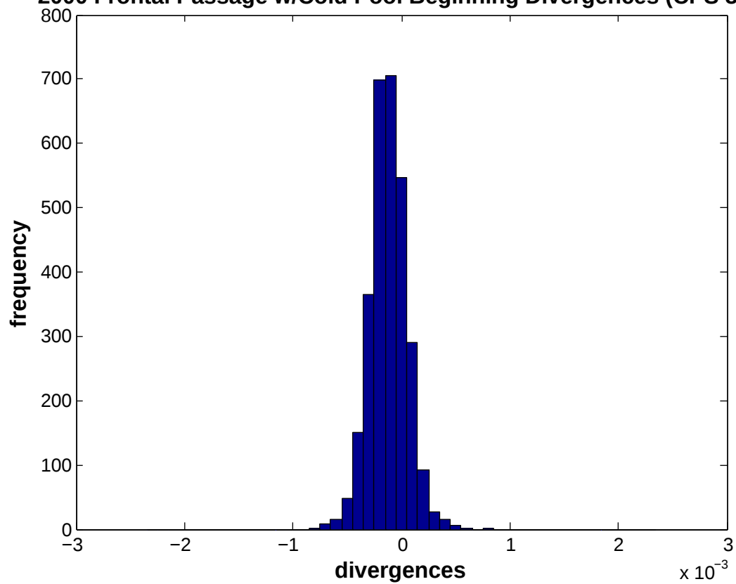
2000 Frontal Passage w/Cold Pool Beginning Divergences (CPS 3+)
