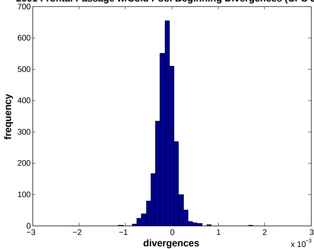
2001 Frontal Passage w/Cold Pool Beginning Divergences (CPS 3+)
