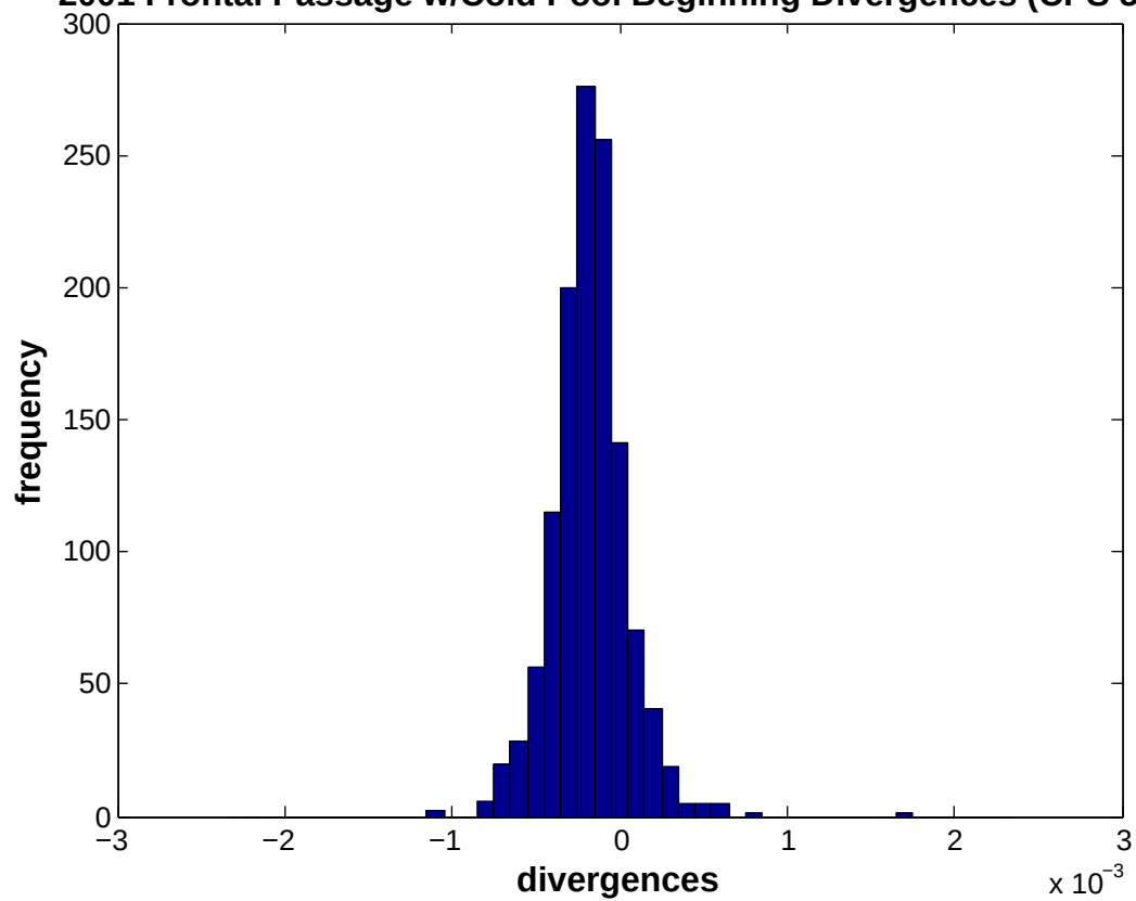
2001 Frontal Passage w/Cold Pool Beginning Divergences (CPS 5+)
