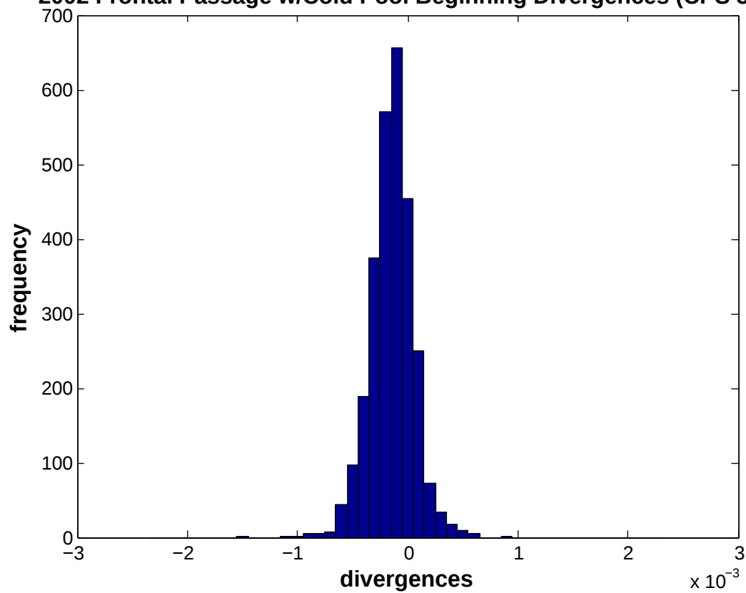
2002 Frontal Passage w/Cold Pool Beginning Divergences (CPS 3+)
