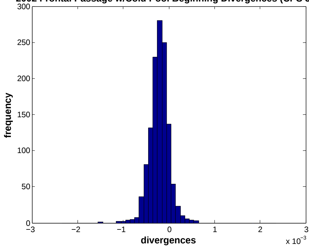
2002 Frontal Passage w/Cold Pool Beginning Divergences (CPS 5+)
